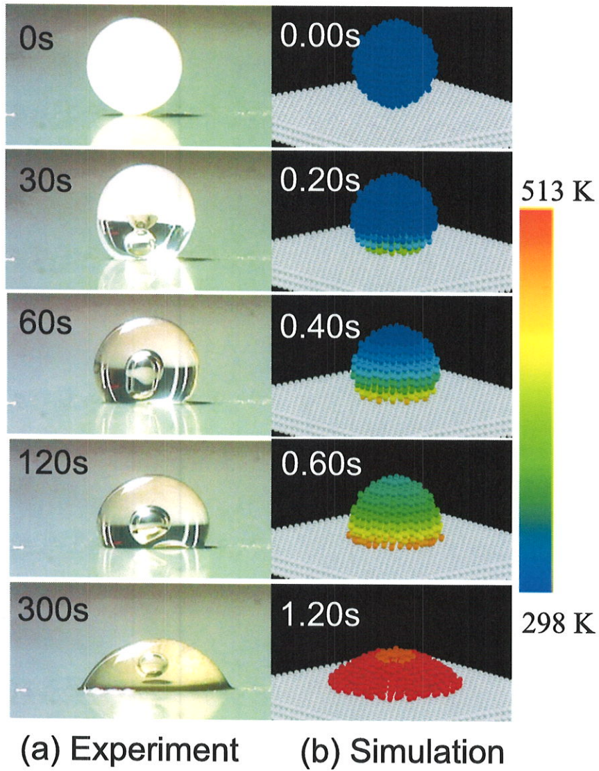
Fig. 5 Melting behavior of polyethylene particle ( D_p=3.2 mm, at 513 K )
